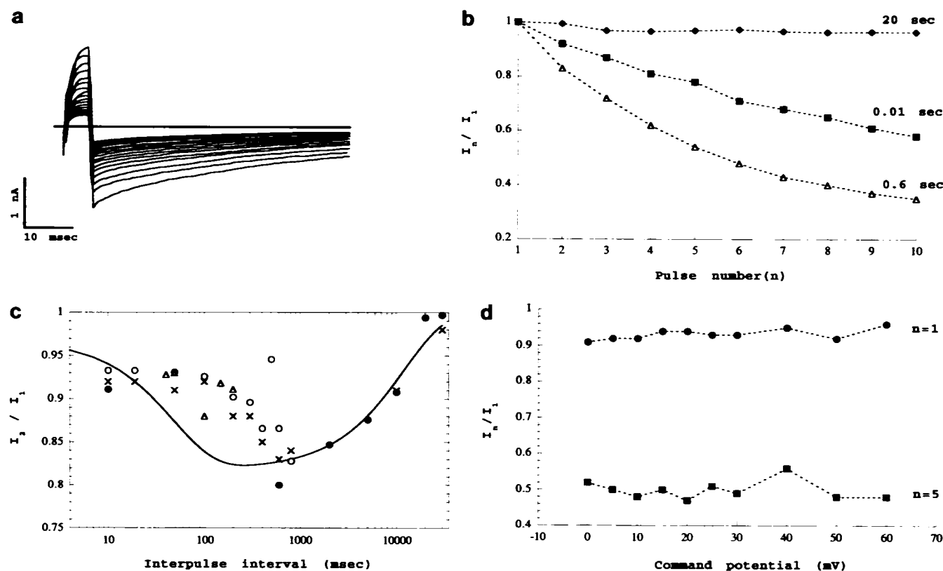
FIGURE 1 Cumulative inactivation of Kv3. (a) Superposition of current traces evoked by a series of 20 5 ms duration pulses to +40 mV, separated by inter-pulse intervals of 50 ms at -80 mV. (b) Frequency dependence of cumulative inactivation. The ratio of the peak current amplitude during each pulse, relative to that during the 1st pulse, is plotted against the pulse number ( n ) at three different inter-pulse intervals (next to each curve). Holding voltage -100 mV, inter-pulse voltage -80 mV, pulse duration 10 ms. (c) Biphasic recovery from inactivation. I_2/I_1 at different inter-pulse intervals from four different patches. Note the logarithmic time scale. The solid line is the prediction of the final model, which is presented and discussed later in the text. (d) Rate of cumulative inactivation is independent of membrane potential during the pulse, as measured by the ratio of I_2/I_1 and I_3/I_1 at several fully activating voltages. Inter-pulse interval 30 ms, pulse duration 30 ms, holding potential between pulses and pulse series is -100 mV.
