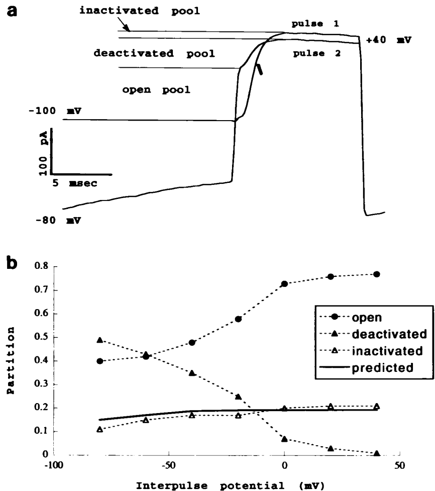
FIGURE 3 Partitioning of channels between open, deactivated, and inactivated pools. (a) The membrane is held at -100 mV for at least 1 min, after which two pulses are delivered to the patch 20 ms apart. Channels that did not deactivate or inactivate during the interpulse interval (open pool) remain open, and they switch current flow direction instantaneously when the membrane potential is changed. Channels that deactivated during the interpulse interval (deactivated pool) show typical activation kinetics, and they peak to a level that is less than the maximum of the first pulse. The difference between the peak currents is the inactivated pool. (b) Partitioning of channels among the three pools, measured as demonstrated in a, as a function of interpulse potential. The probability of finding a channel in the inactivated pool declines monotonically with more hyperpolarized interpulse voltages. Pulse duration 5 ms, interpulse interval 50 ms. The solid line is the behavior of the inactivated pool as predicted by the final model, which is presented and discussed later in the text.
