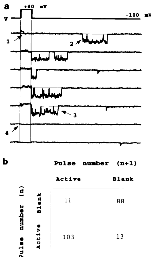
FIGURE 7 Channel reopening upon recovery from the inactivated state during the interpulse interval. ( a ) Each sweep contains a 20-ms pulse to +40 mV, followed by an inter-pulse interval of 200 ms. Each experiment includes 25 sweeps (the figure contains seven consecutive sweeps from one representative experiment). Data are sampled continuously throughout each experiment. Arrow #1 depicts inactivation during a pulse; a reopening event during the interpulse is marked by arrow #2; channel inactivation during the interpulse interval is marked by arrow #3; and the beginning of a blank cluster is shown by arrow #4. The V-shaped current glitches seen in traces 3, 5, and 7 are caused by a discharge of head-stage capacity. ( b ) Clustering of active and blank traces, classified as described in a . Analysis was done by visual inspection of each individual trace, marking it as a blank if no channel opening was observed throughout the trace. Note the strong correlation between the activity at pulse number n and the activity at pulse number (n + 1) .
