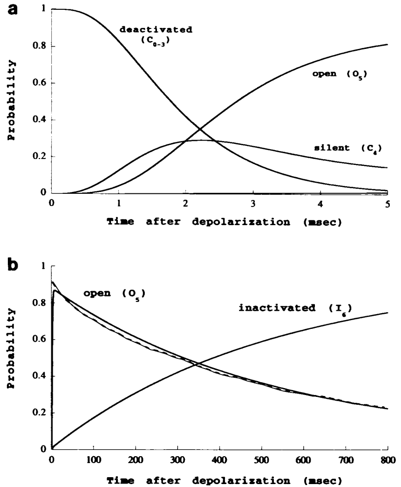
FIGURE 8 A numerical simulation of Scheme 7. Initial conditions: C_0 = 1.0 , V_{\text{command}} = +40 mV. Activation and deactivation rate equations as described in Fig. 5. k_{46} = 0.025 \text{ ms}^{-1} ; k_{54} = 0.0001 \text{ ms}^{-1} ; k_{45} = 1.2 \text{ ms}^{-1} ; k_{54} = 0.15 \text{ ms}^{-1} . (a) Expansion of the first 5 ms. (b) Longer time scale. The dashed line represents mean normalized current decay during long pulse inactivation ( \tau = 811 ms, SD = 147, n = 3 ).
